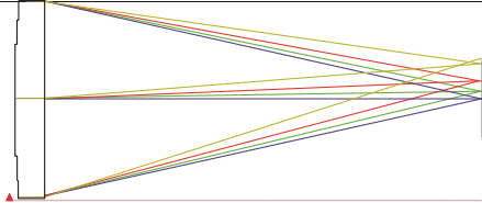
Figure 1. Layout of the refractive lens.
