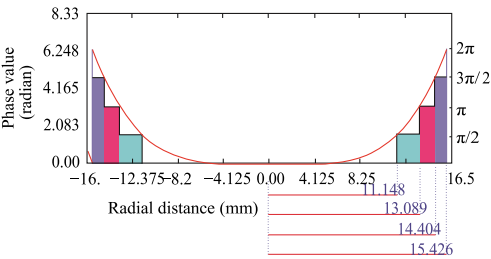
Fig.ure 3: Phase curve versus aperture of the diffractive surface sliced into 2π layers and the discrete phase levels.
