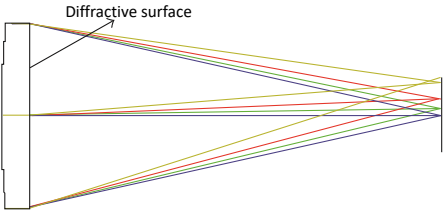
Fig.ure 2: Layout of the diffractive lens.
